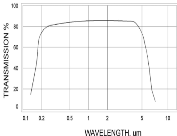
Sapphire zero length transmission curve
