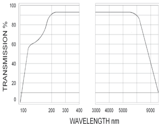
Magnesium fluoride transmission curve
